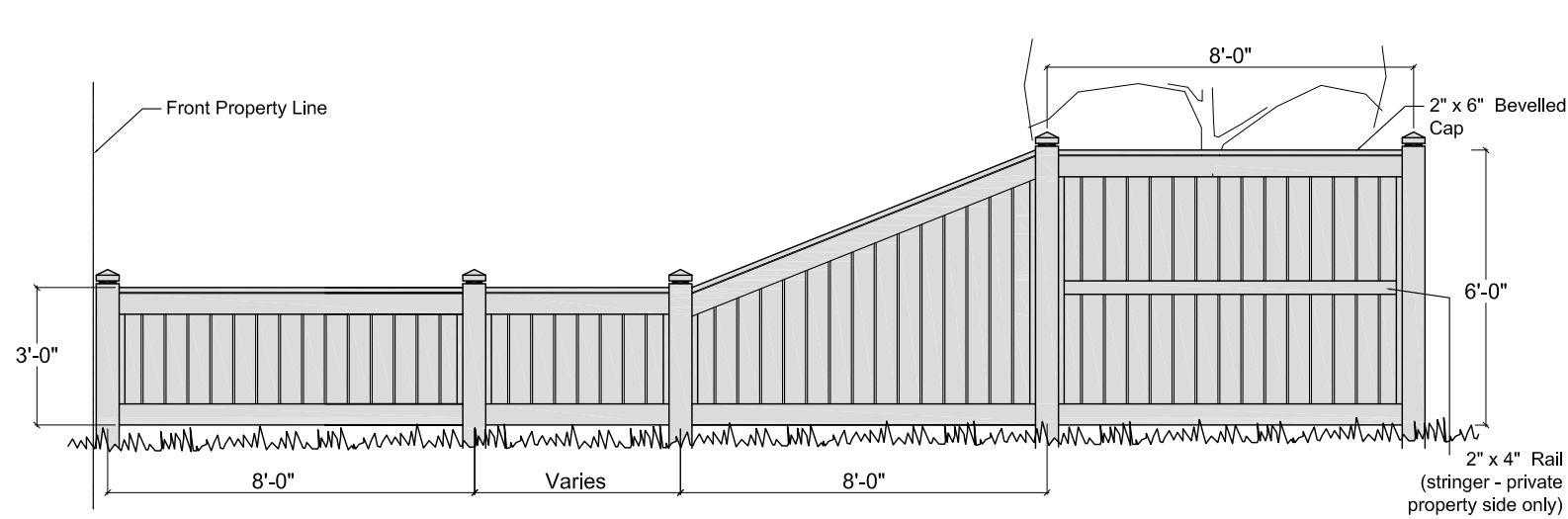
2 Solid Fence - Street or Path Side Yard - Typ. 9BW Solid Fence along Side Yard Design - NTS
