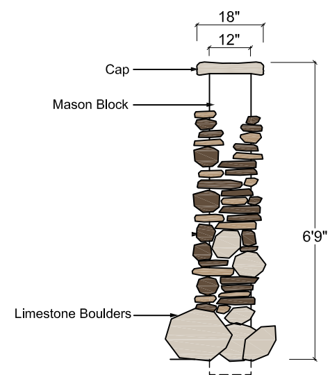
5 Pillar Elevation - Typ. 9BW Corner Pillar Detail on Berm - NTS
