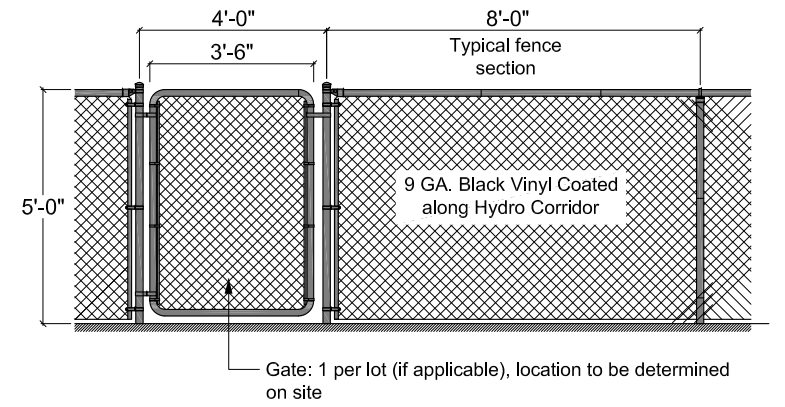
3 Rear Yard Chain-link Fence Elevation - Typ. 9BW Chain-link Fence Design - NTS
