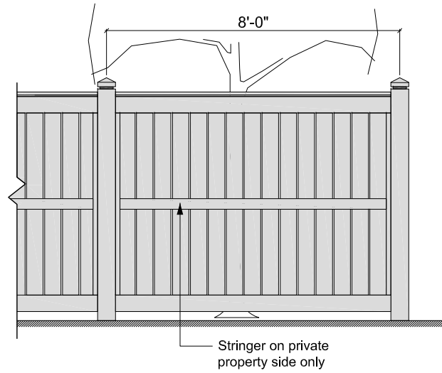
1 Solid Fence Elevation - Typ. 9BW Solid Fence Design - NTS
