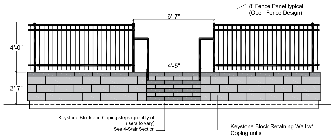
4 Front Yard Retaining Wall Elevation - Typ. 9BW Open Fence w/ Retaining Wall - NTS
