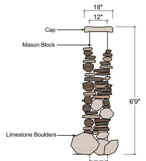
5 Pillar Elevation - Typ. 9BW Corner Pillar Detail on Berm - NTS
